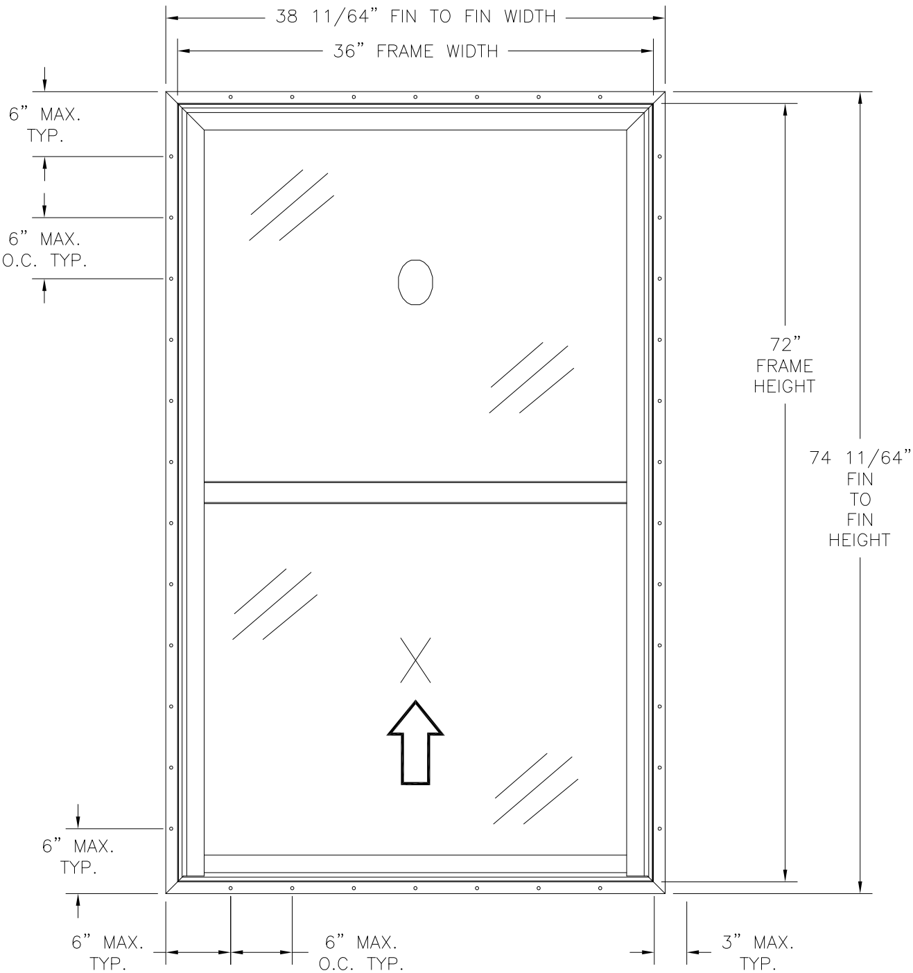
SHORELINE 1100 SH PVC SINGLE HUNG WINDOW EXTERIOR VIEW
